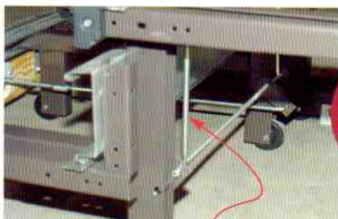
Interkal Quality: Continuous Vertical Engagement Rods provide positive engagement into the continuous locking angle at both front and rear.
